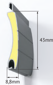
Lame Isolante 43 Shutter Slats with isolation 43
